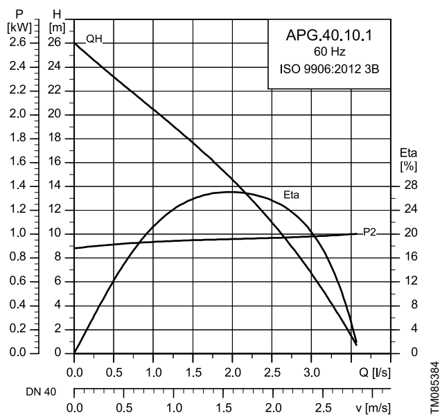
UNILIFT APG, single-phase motor
