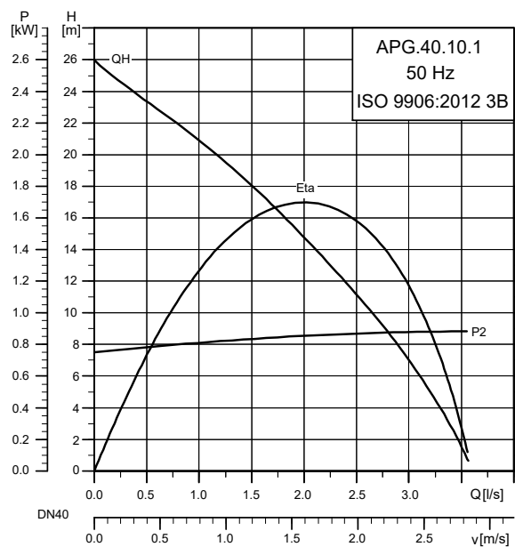
UNILIFT APG, single-phase motor
